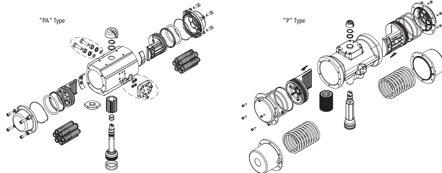
"P" type pneumatic servomotor
