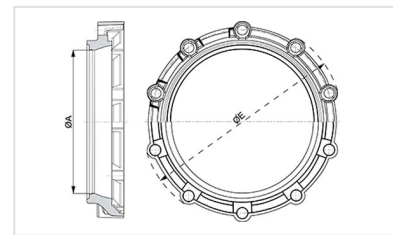
Gland for STD Ve joint DN80-1200
