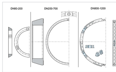
Locking ring for STD Ve joint DN80-1200
