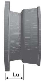
EXP - DN 60 to 300
