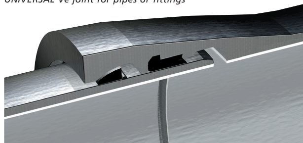
UNIVERSAL Ve joint for pipes or fittings
