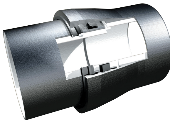
UNIVERSAL Vi joint for pipes or fittings
