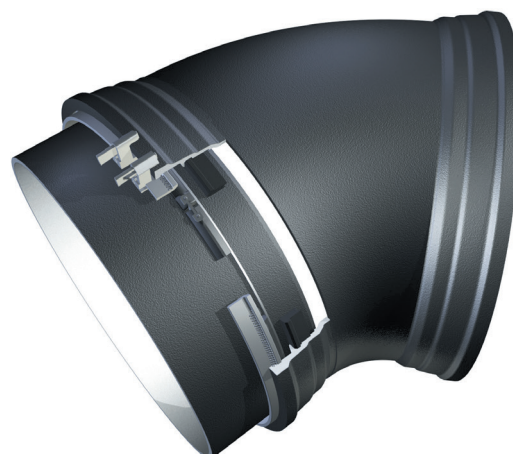
PAMLOCK joint for pipe or fittings
