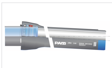
Ensemble Tuyau universel Standard ZMU + Joint Universal Standard Vi
