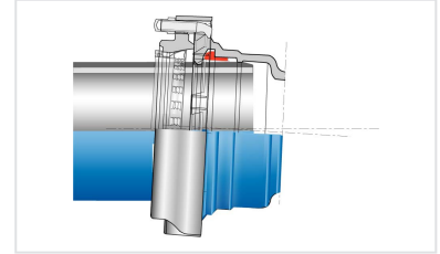
Ensemble Raccord Standard PECB + Joint Standard V+i
