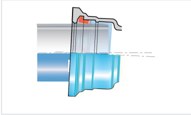
Ensemble Coude Standard PECB + Joint Standard
