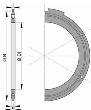
Gasket DN40 to DN300
