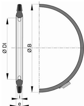
Gasket with metallic inserts DN350 to 2000
