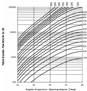
VALVOLA A FARFALLA - BUTTERFLY VALVE
