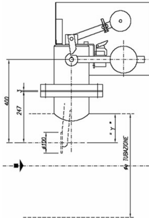
Version for manual resetting pump
