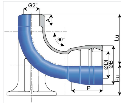
With Socket threaded 2" Gas
