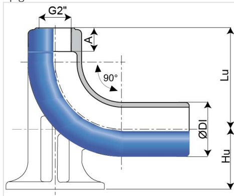
With Spigot threaded 2" Gas
