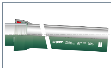
Kit Standard IRRIGAL pipe + Standard Gasket
