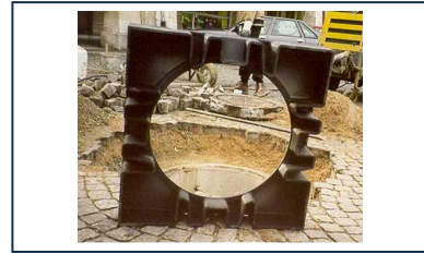
Manhole cover PAMREX 600 - D400 class - Installation of the manhole cover with apparent frame
