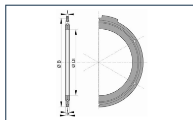
Flanged joint with metallized steel bolts and nuts
