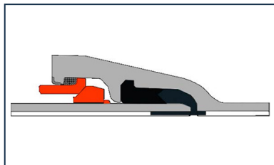
Kit PAMLOCK Fitting PECB + PAMLOCK Joint
