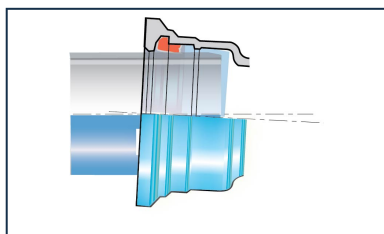
Kit Standard Flanged Socket PECB + Standard Gasket
