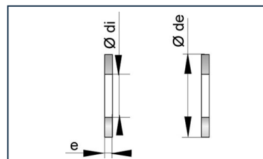
Galvanised Steel Washers for Bolts
