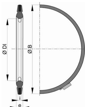
Gasket with metallic inserts DN350-2000 EPDM
