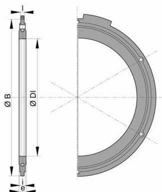
Gasket with metallic inserts DN350 to 2000
