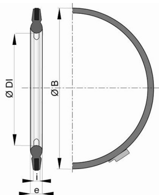
Gasket with metallic inserts DN350 to 2000
