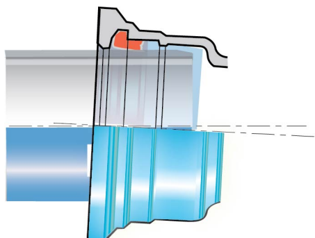
Mobile flange
