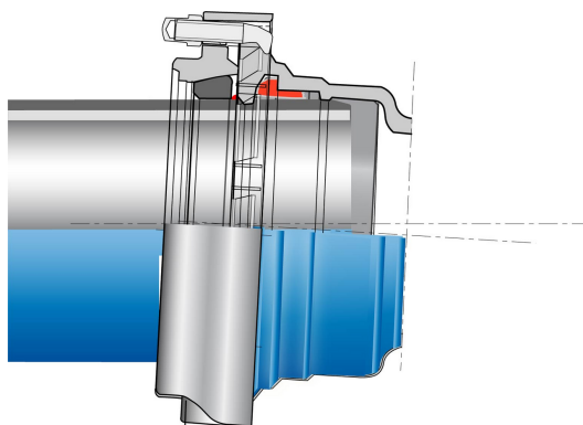
Standard Double Socket Bends
