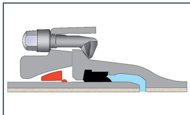
STD Ve joint for fittings DN80-1200
