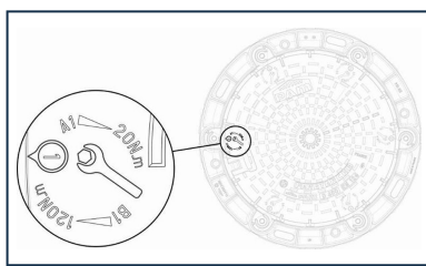
Manhole cover PAMTIGHT - D400 class - Disassembling/ Reassembly of the cover
