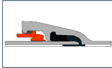
PAMLOCK joint
