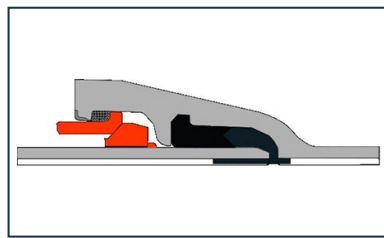
PAMLOCK joint
