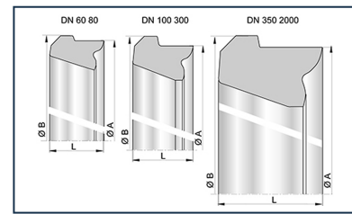
Standard gasket for Pipes and Fittings DN60-2000
