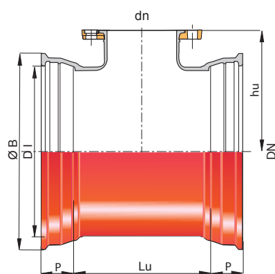
DN 700 to 2000
