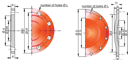
DN 1100 to 2000
