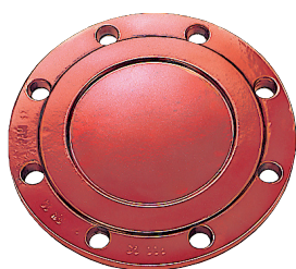
DN 700 to 1000
