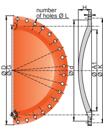
DN 1100 to 2000
