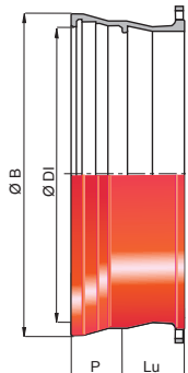
DN 700 to 2000
