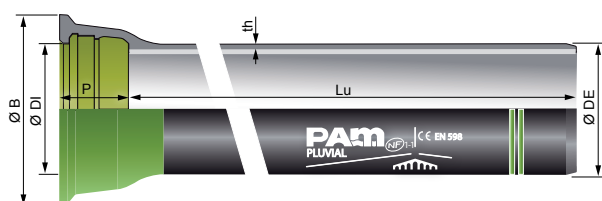
DN 350 to 1200
