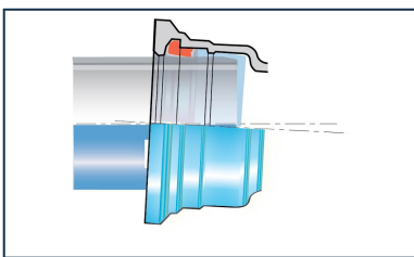
Kit Standard Taper PECB + Standard Gasket
