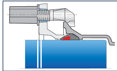
Kit Express Fitting AQB + Express Vi Gasket
