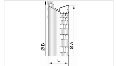
UNI Vi Locked Ring DN80-700
