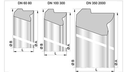
Standard gasket for Pipes and Fittings DN60-2000
