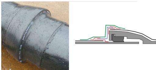
Assembly of the aluminium sleeve on TT pipes
