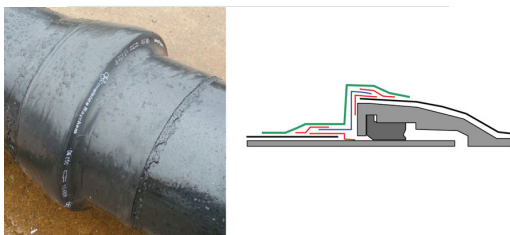
Assembly of the aluminium sleeve on TT pipes
