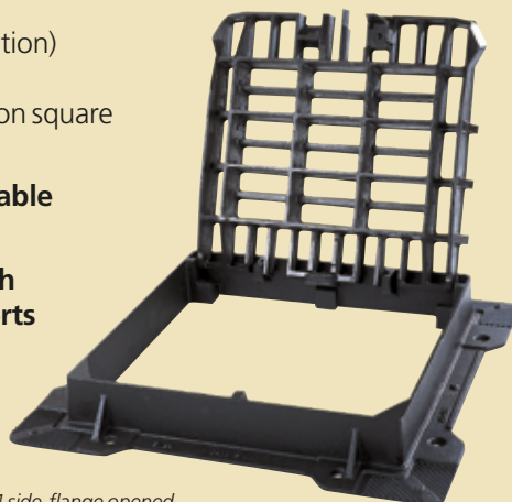
→ Frame 4 side-flange opened
