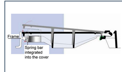
Manhole covers - Locking of the cover by spring bar
