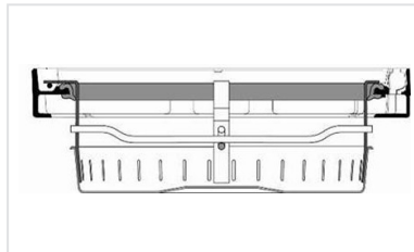
Mudpan for VIATOP/ DYNATOP Manhole covers
