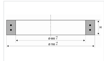
Concrete Ring for VIATOP 600 NIVEAU Manhole cover
