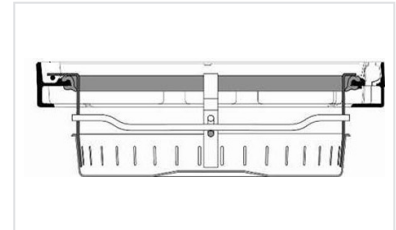
Mudpan for VIATOP/ DYNATOP Manhole covers
