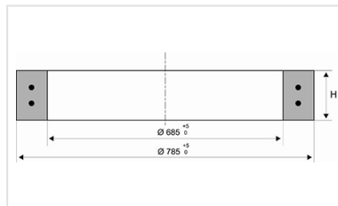
Concrete Ring for VIATOP 600 NIVEAU Manhole cover
