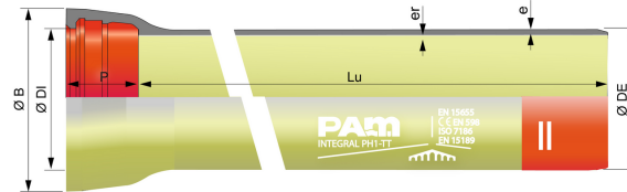
Pipe without collerette DN150-1000
