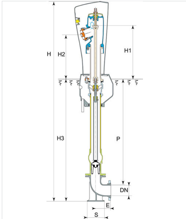
Straight valve box
