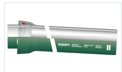
Kit Standard IRRIGAL Pipe + Standard Vi Gasket
