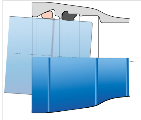
Angular deflection
