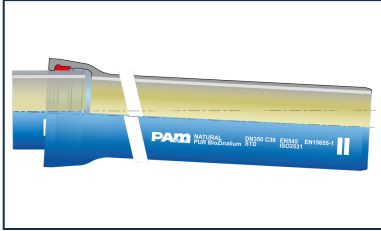
Kit Standard PUR Pipe + Standard Gasket
