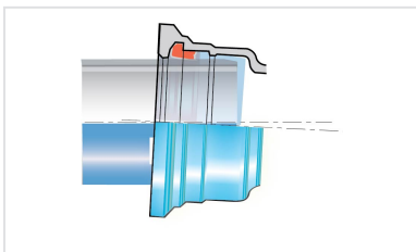
Kit Brida Enchufe Standard PECB + Junta Standard
