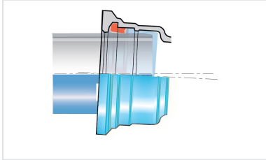
Kit Codo Standard PECB + Junta Standard
