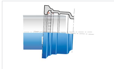
Ensemble Raccord Standard AQB + Joint Standard Vi
