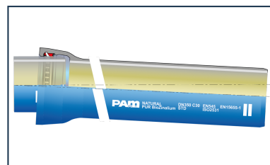
Ensemble Tuyau Standard PUR + Joint Standard Vi
