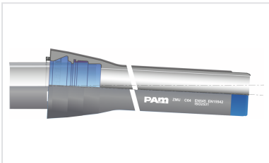
Ensemble Tuyau Universel Tyton ZMU + Joint Universel Tyton Vi
